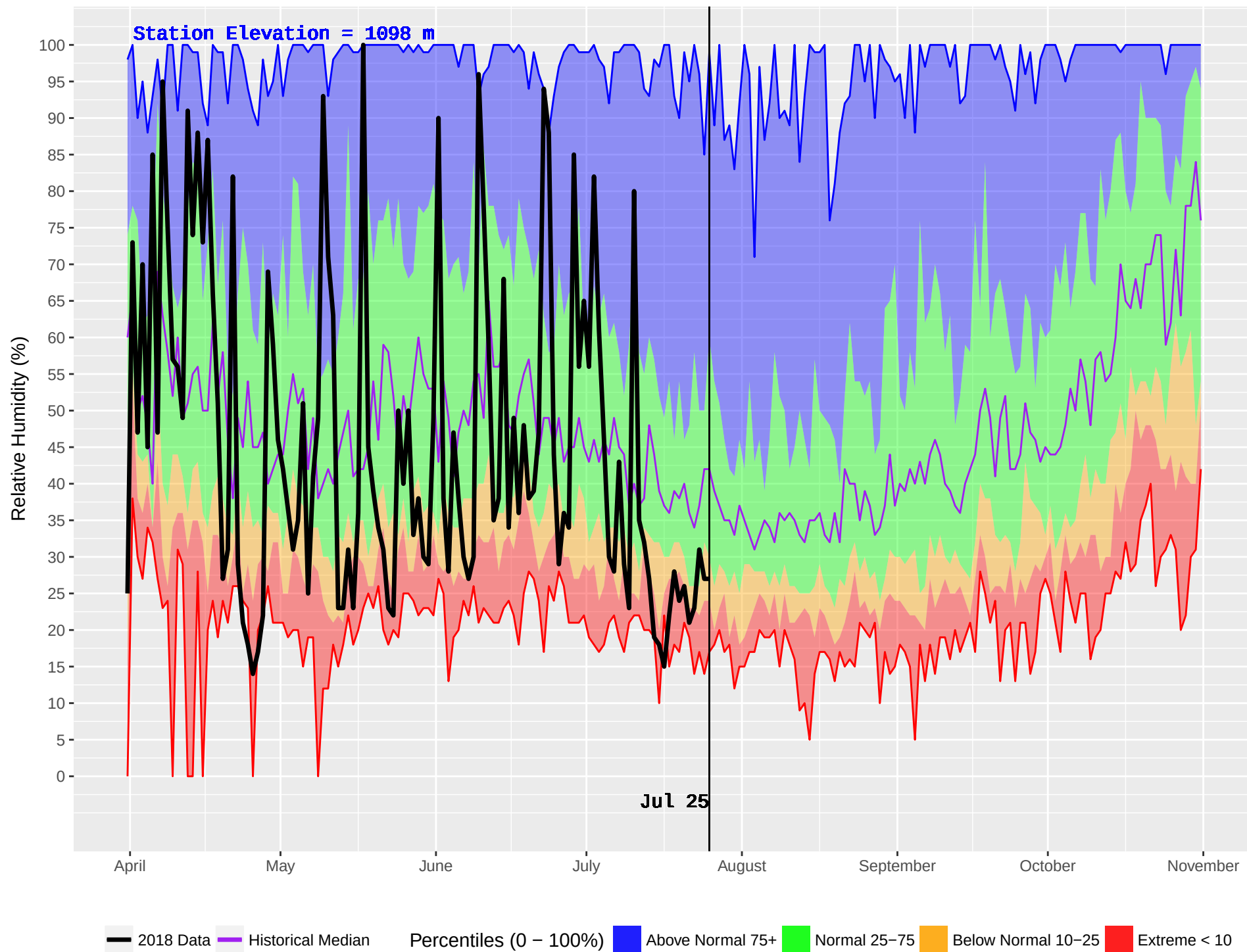
GOATFELL (401) : Historical (1986–2016) and Current (2018) Noon Relative Humidity
