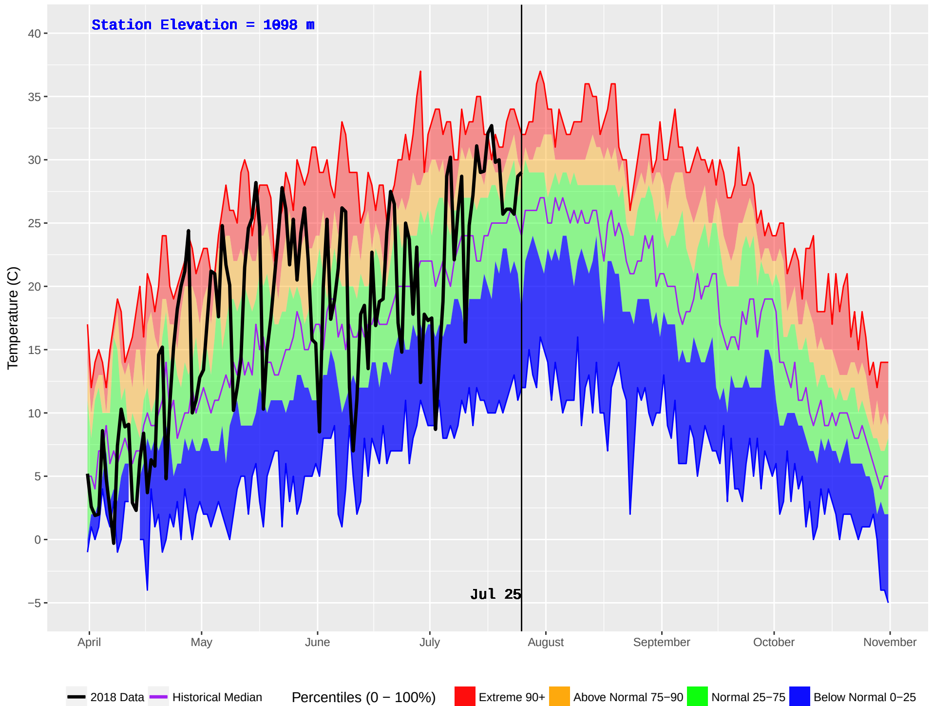
GOATFELL (401) : Historical (1986–2016) and Current (2018) Noon Temperature
