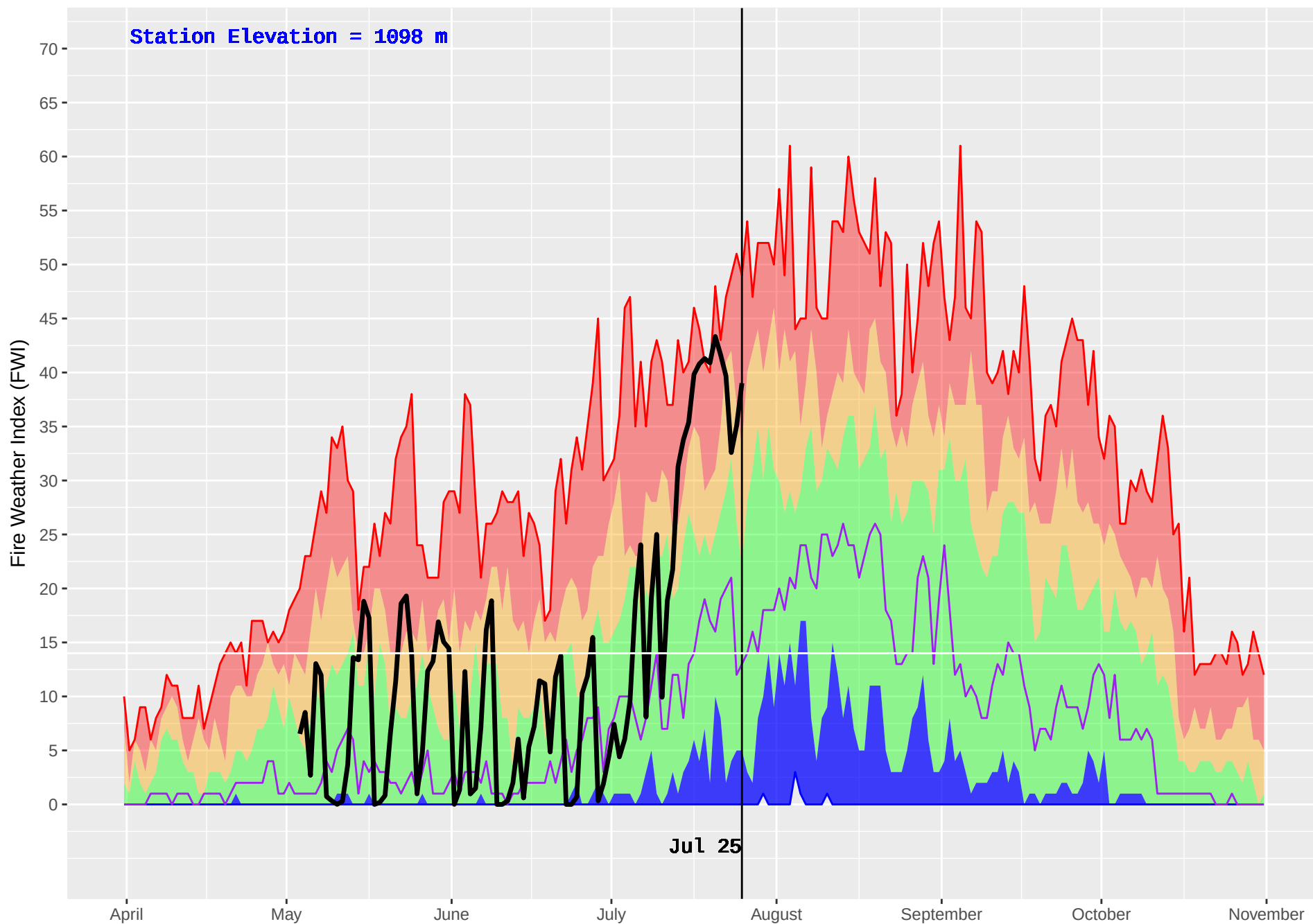
GOATFELL (401) : Historical (1986–2016) and Current (2018) Noon Fire Weather Index (FWI)
