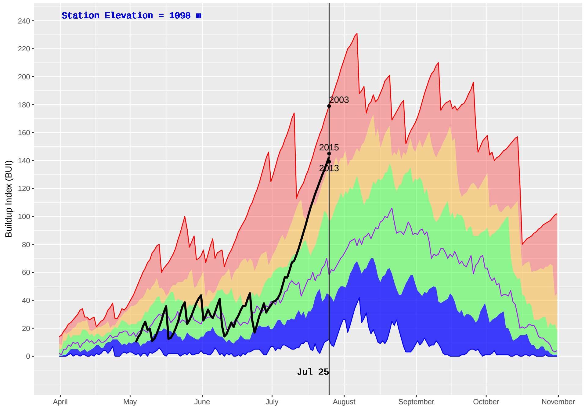
GOATFELL (401) : Historical (1986–2016) and Current (2018) Noon Buildup Index (BUI)
